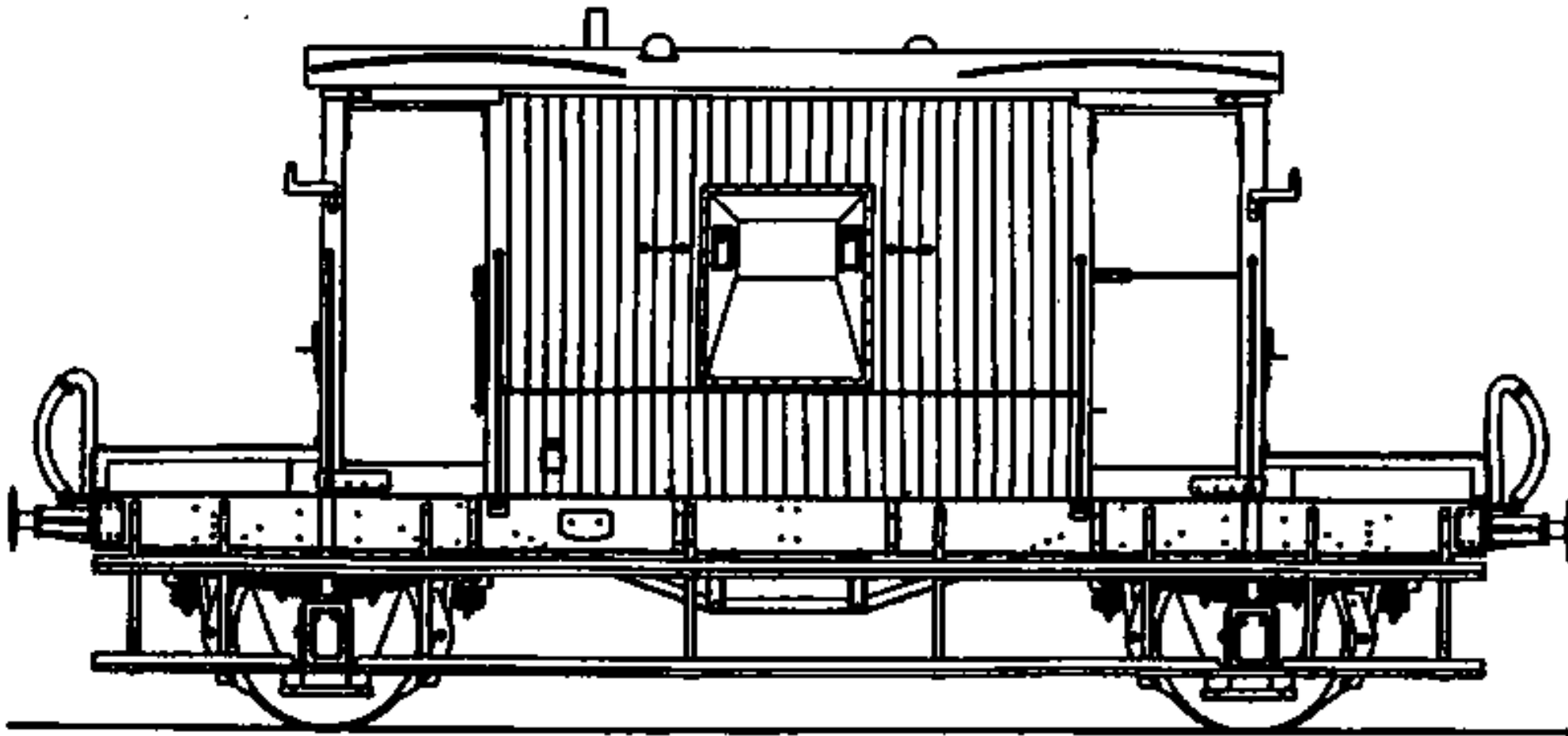
BRITISH RAILWAYS STANDARD BRAKE VAN BUILT 1951 No. B951144 WEIGHT 20 ton LENGTH 27'
